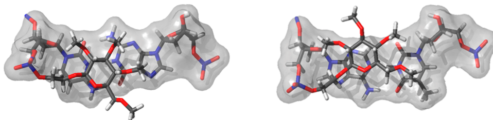
Figure 2. Top view of self-complementary DNA conjugates forming a double helix, permethylated glucose– \text{CH}_2\text{CH}_2-\text{OPO}_2^--\text{CGCGCG} (left) and permethylated glucose– \text{CH}_2\text{CH}_2-\text{OPO}_2^--\text{AGCGCT} (right). The apolar carbohydrate stacks on top of a C–G base pair (left) and the apolar carbohydrate stacks on top of an A–T base pair (right).
